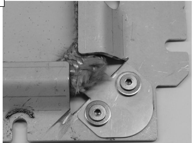
Figure 15: Glass-frame clips
