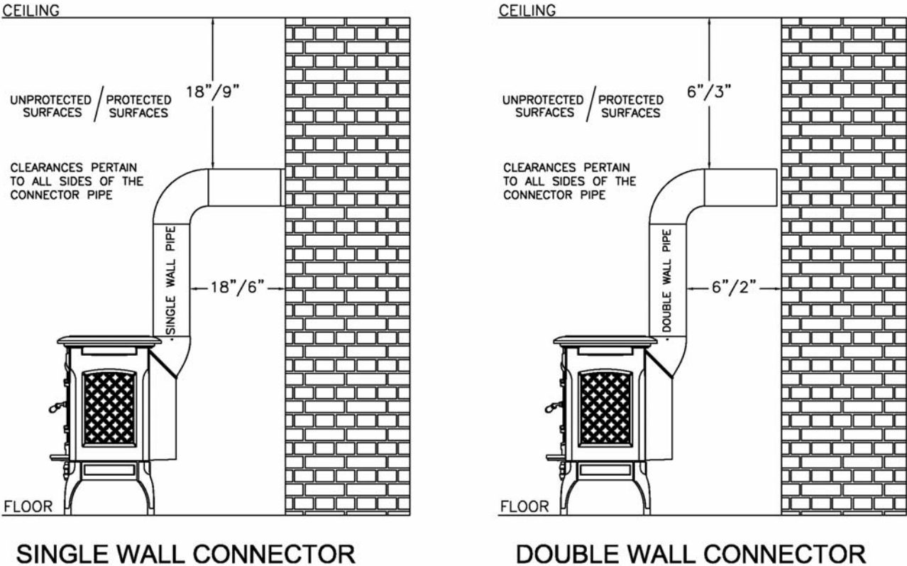
Figure 7 – Connector Clearances
