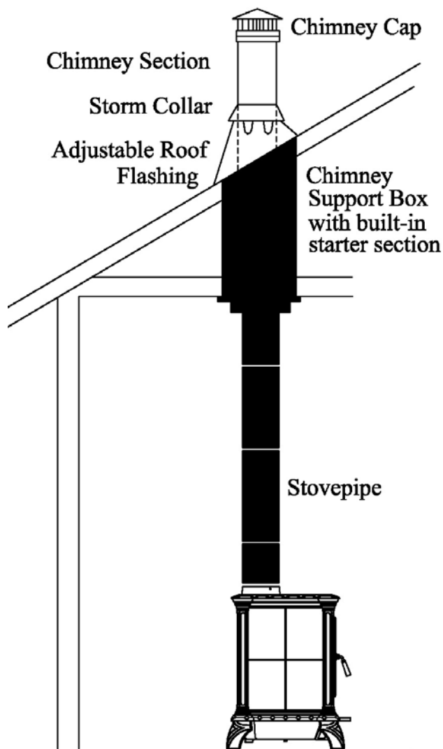
Typical Mobile Home installation. Chimney supported by ceiling.
