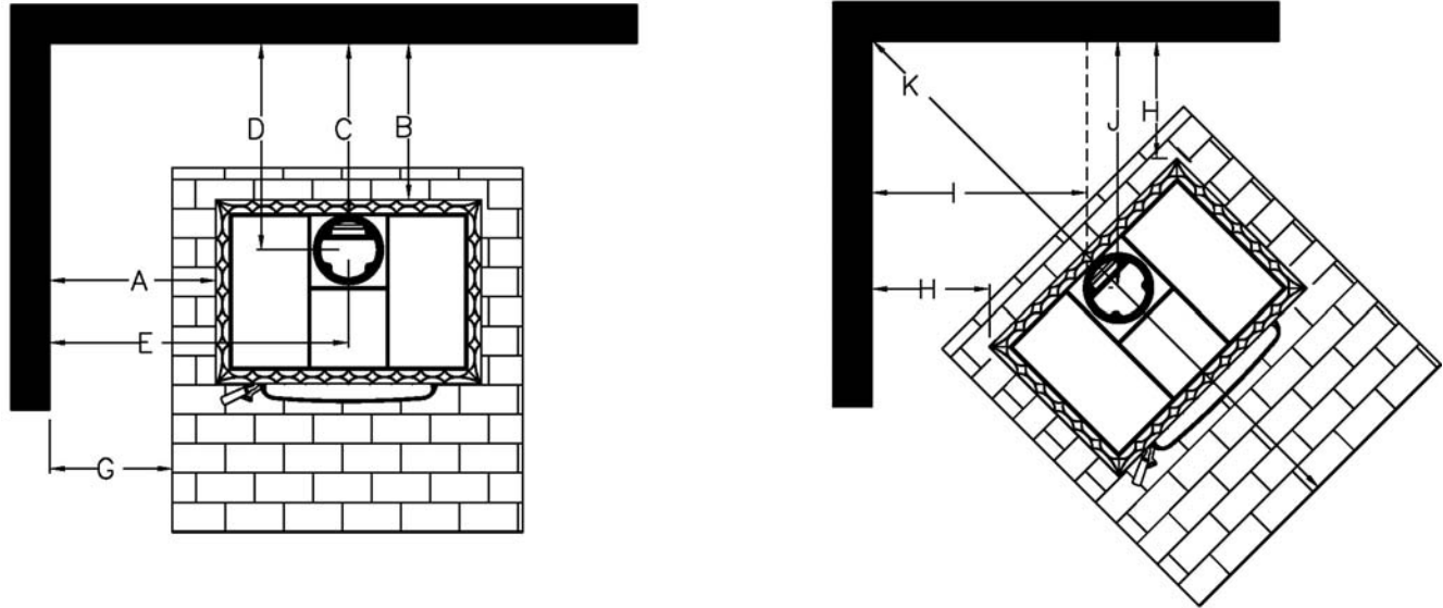
Figure 4: Tribute 8040 Clearances
