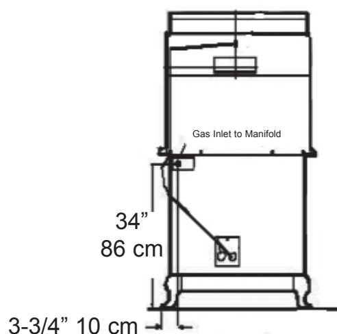
9200 Gas Inlet Locations
