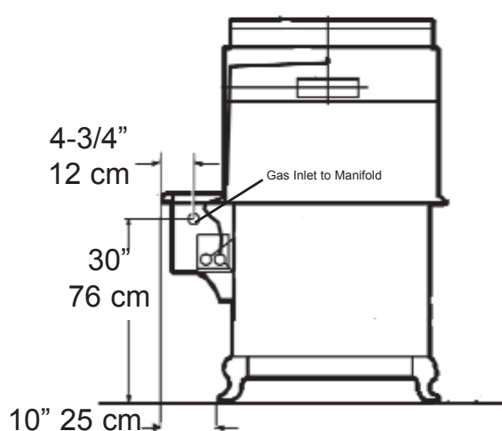
7200 Gas Inlet Locations
