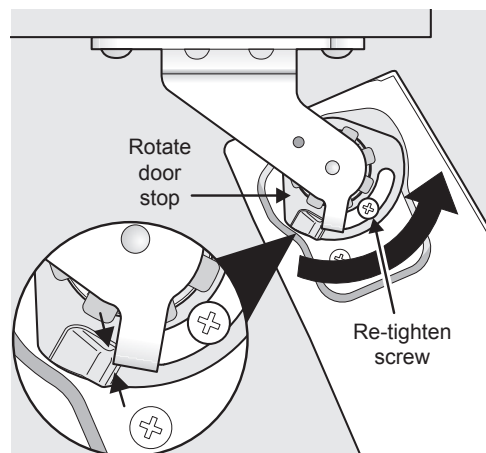
Re-tighten screw
