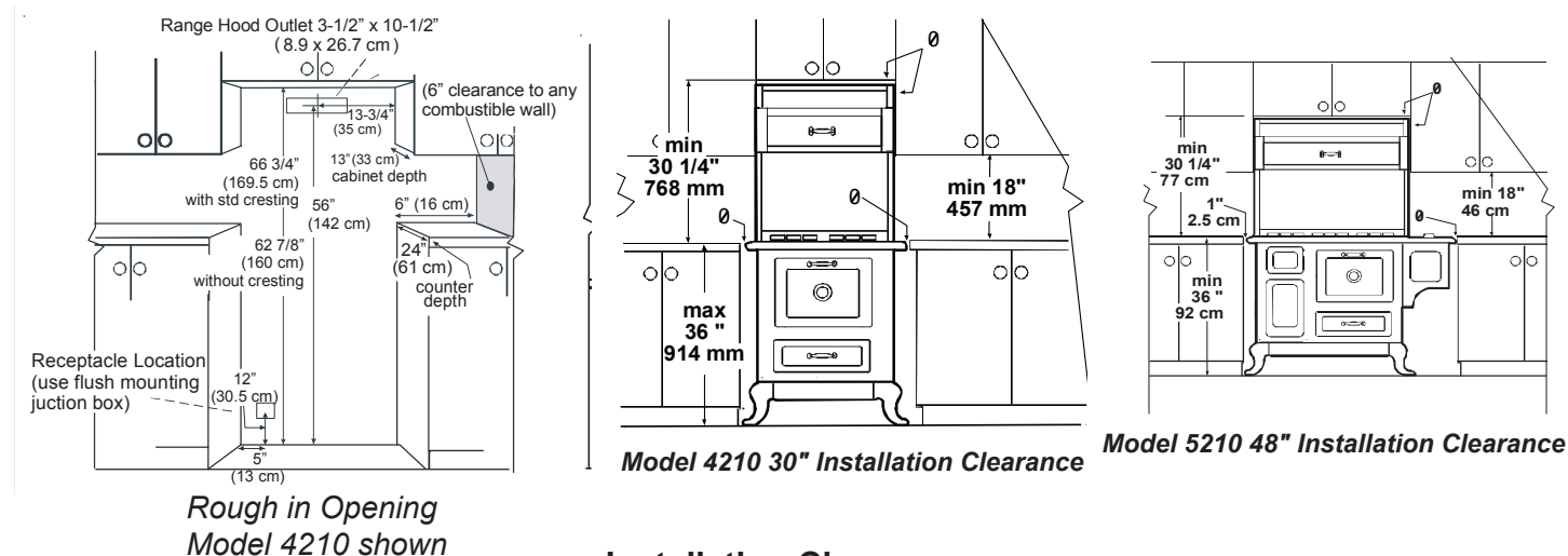
Fig 3 Installation Clearances
