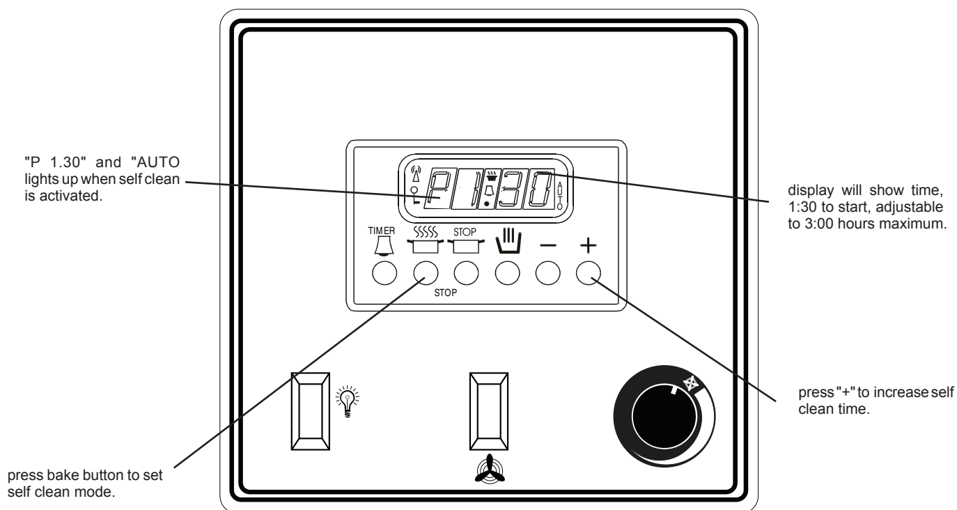
Figure A - Control Panel Layout
