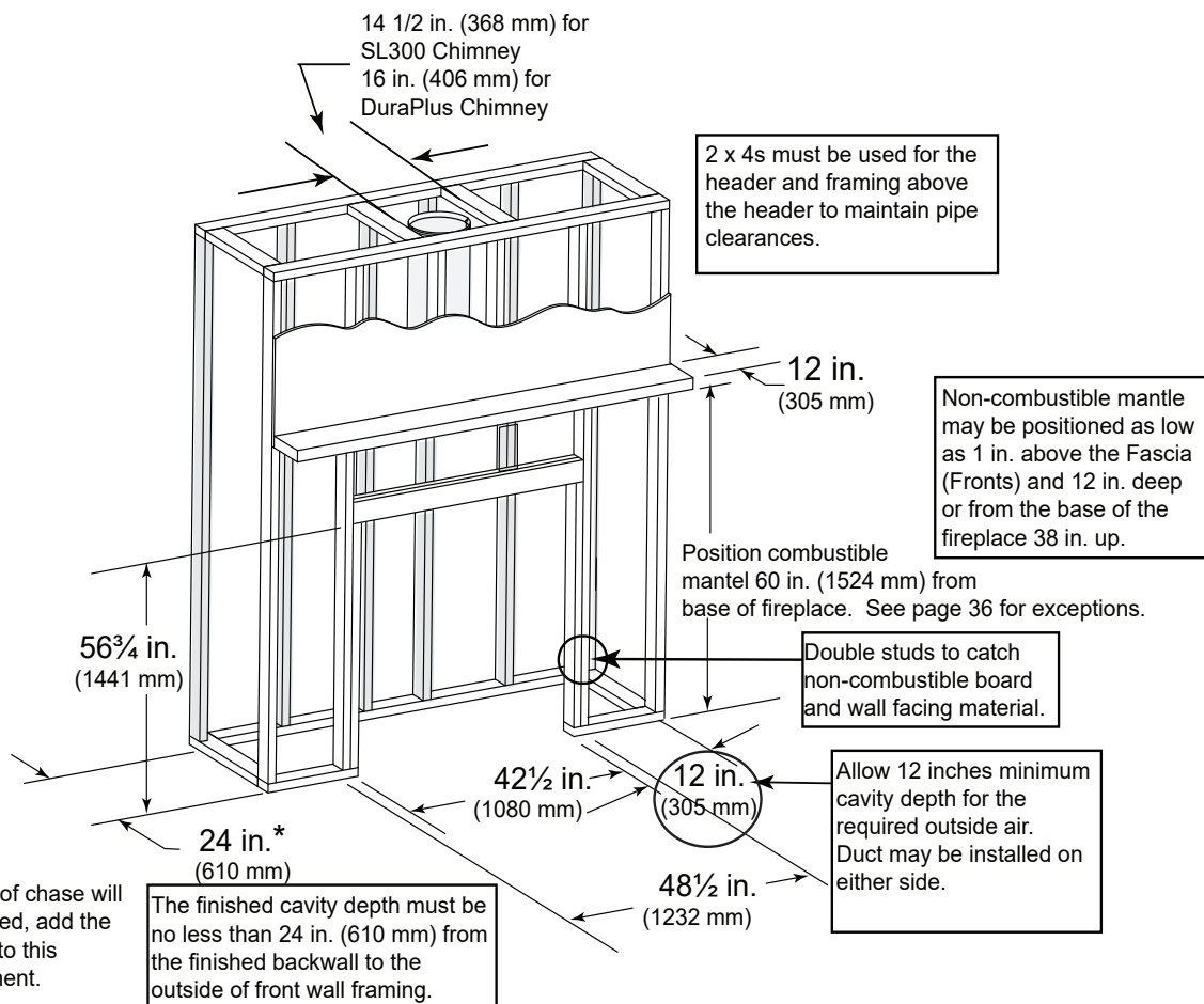
Figure 3.5 Framing the Fireplace
