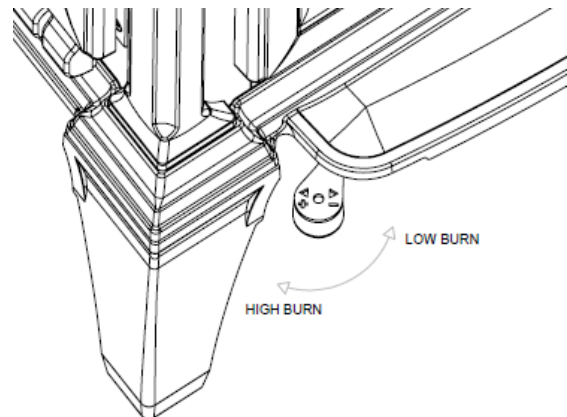
Figure 8 – Air Control
