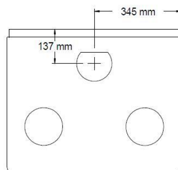
Top view showing position of flue spigot:-
