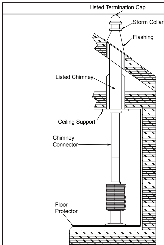
Figure 12.2 - Prefabricated Interior Chimney
