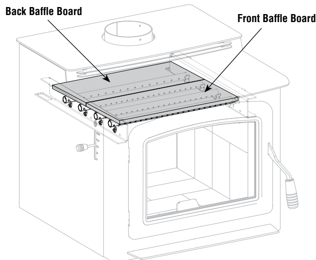
Figure 26 - GV300 Baffle Boards Installed
