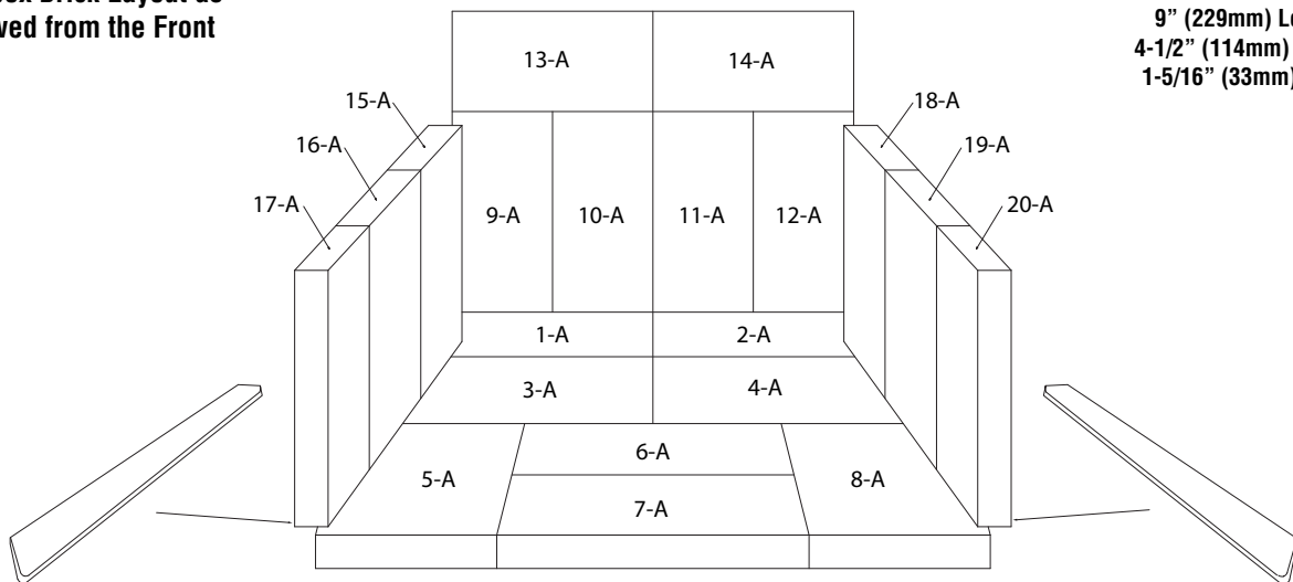
Figure 22 - GV230 Brick Diagram
