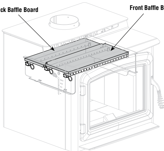
Figure 23 - GV230 Baffle Boards Installed
