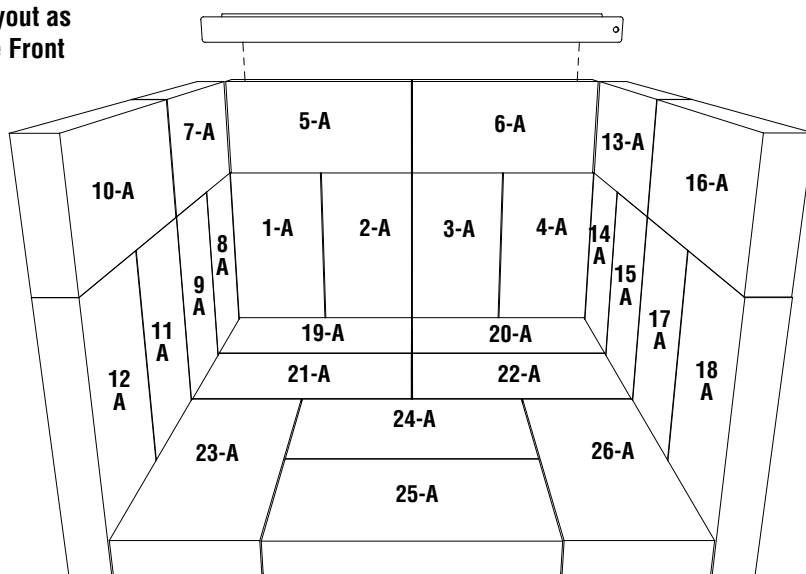
Figure 25 - GV300 Brick Diagram
