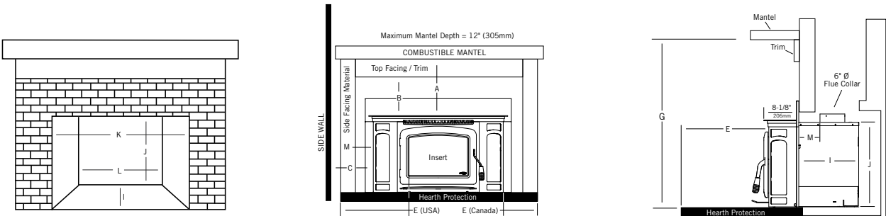
*Illustrations apply to Montlake™
