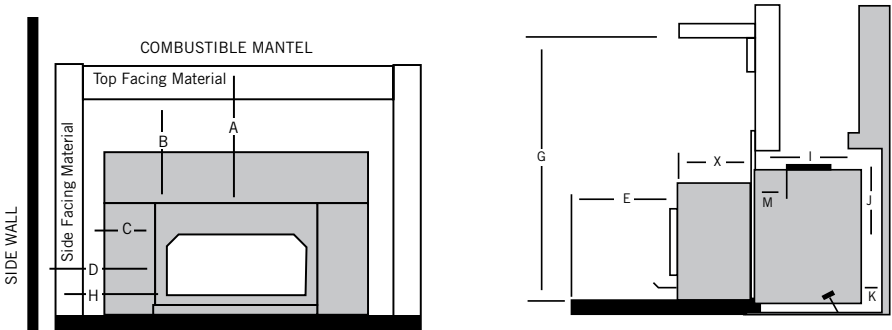
*Illustrations apply to Striker™ C160, Performer™ C210, Legacy™ C260, & Canyon™ C310
