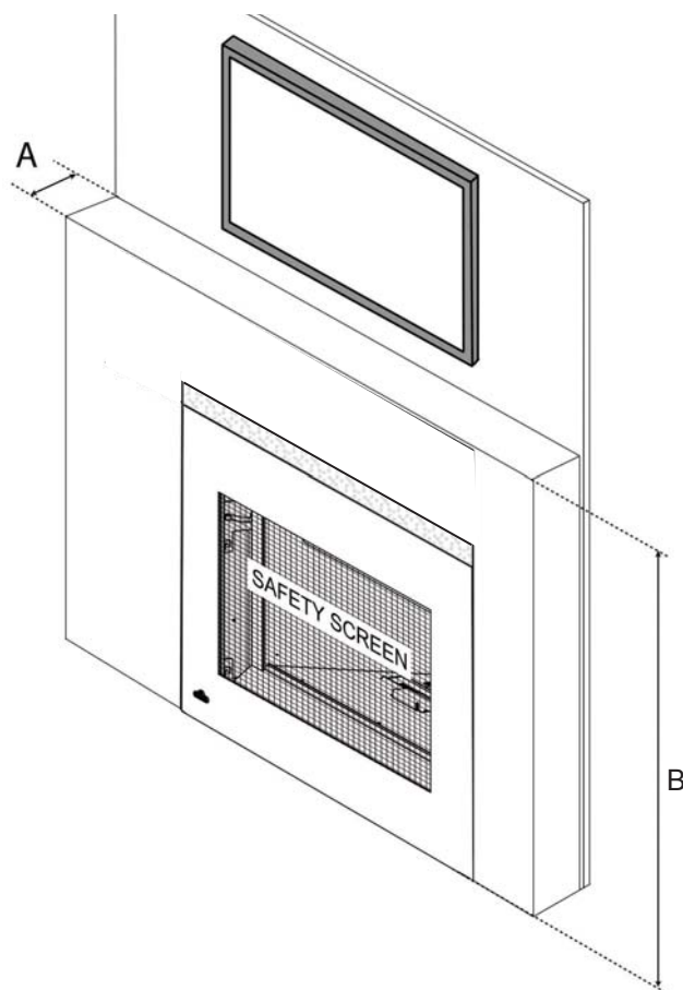
CLEARANCES CHART
