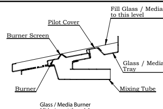
Glass / Media Burner * Side view cut-through *
