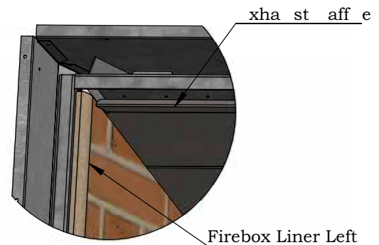
Exhaust Baffle
