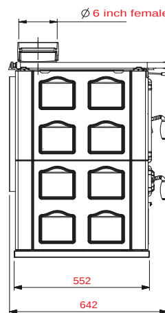
ROSA UL-C Ceramic - 183 kg
