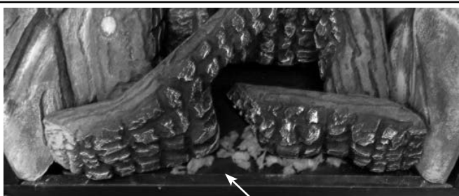
Figure 12 - Ember Placement DO NOT place ember material directly over the ember burner ports.
