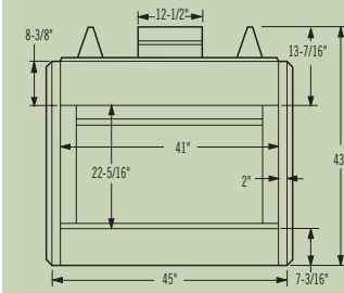
Front View (BR-42 shown)
