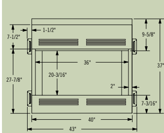
Front View (BC-36 shown)
