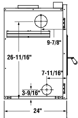
Figure 9 - Fireplace and Framing Dimensions
