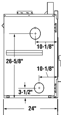
Figure 11 - Fireplace and Framing Dimensions
