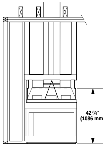
Right Front View
