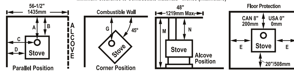
Minimum Clearance to Combustible Materials - Inches (millimeters)
