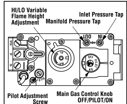
Figure 1 - SIT Millivolt Gas Valve
