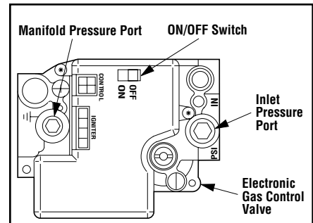
Figure 2 Honeywell Electronic Gas Valve
