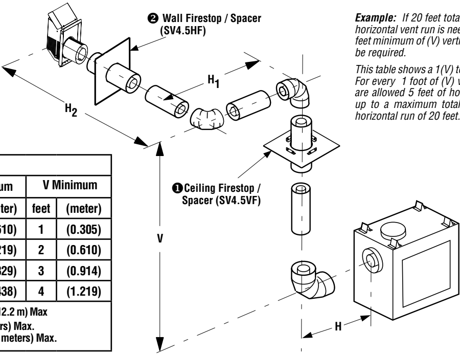
Square termination (SV4.5HT-2) shown Figure 47 - Side Vent, THREE 90 DEGREE ELBOWS
