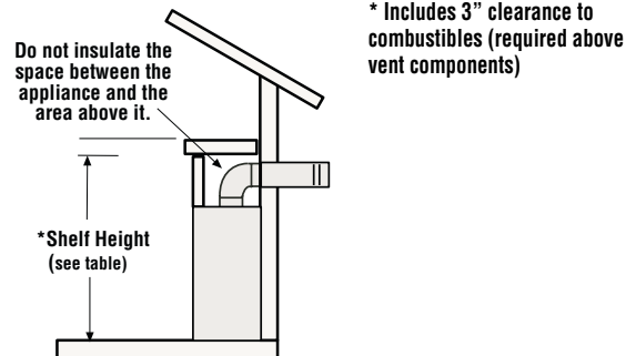
Figure 8 - Shelf Height Minimum Clearances With Top Venting
