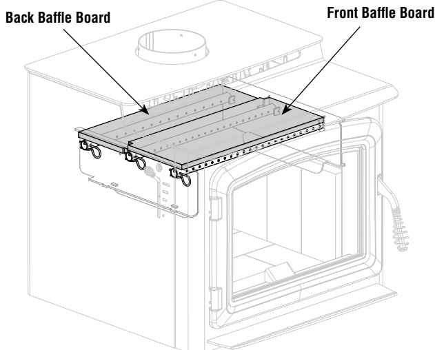
Figure 23 - GV230 Baffle Boards Installed
