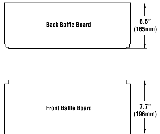
Figure 24 - GV230 Baffle Boards
