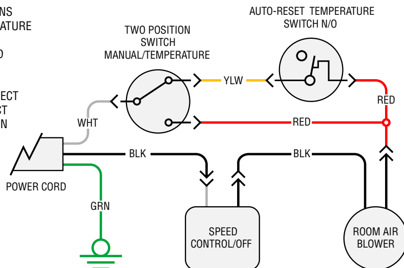
Figure 34 - Blower Wiring Schematic
