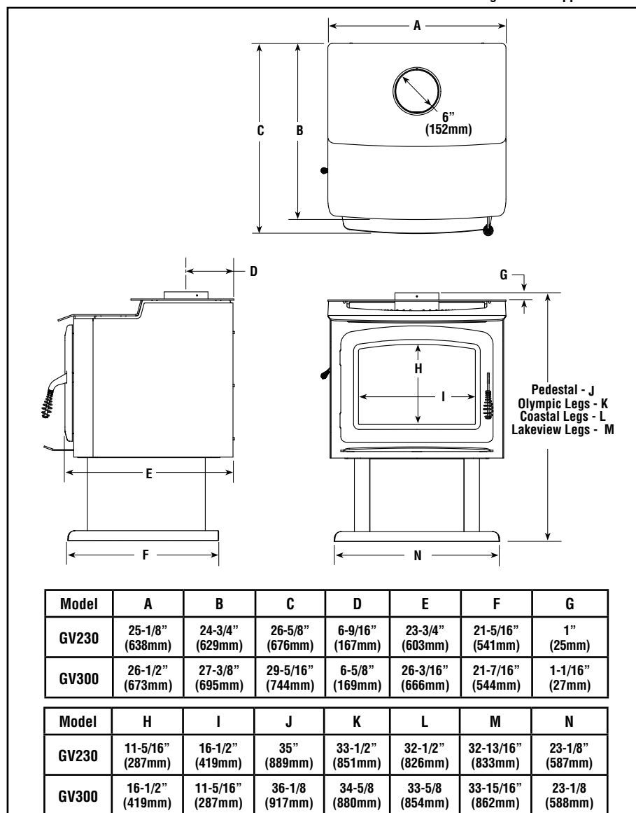
Figure 8 - Dimensions
