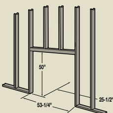
LBR-4324 FRAMING
