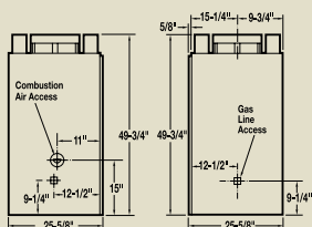
LBR-4324 FRAMING
