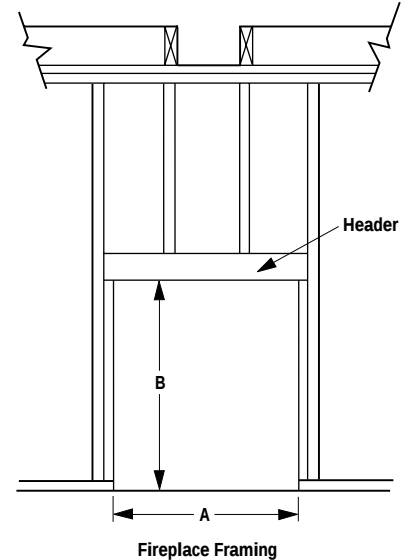
Framing Dimensions
