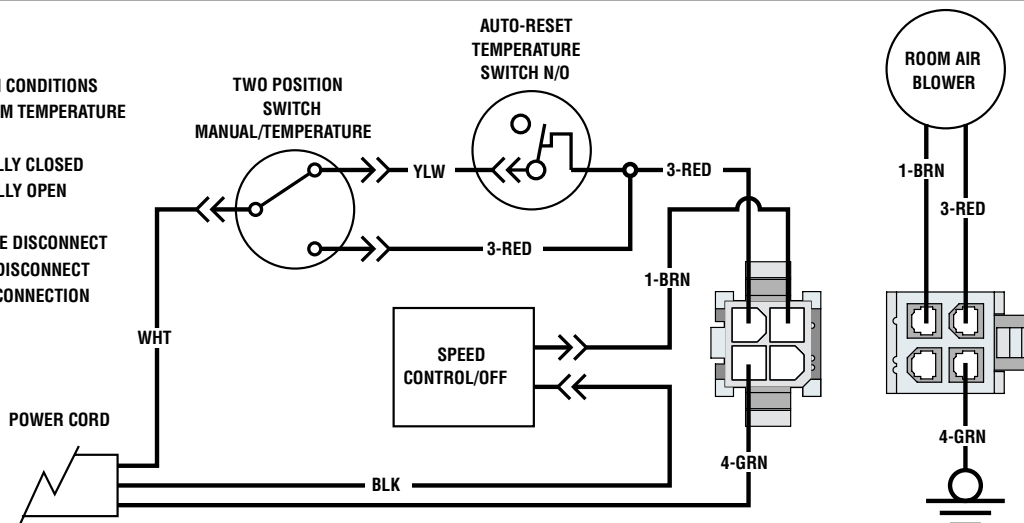
Figure 18 - Blower Wiring Schematic
