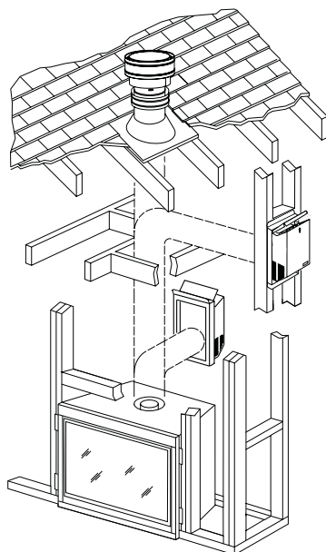
Typical Installation
