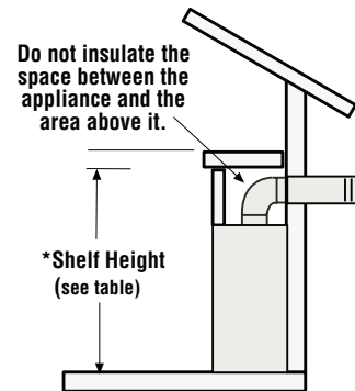
Figure 7 - Shelf Height Minimum Clearances With Top Venting
