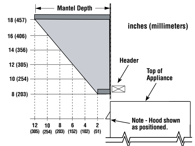
Figure 8 - Minimum Mantel Clearances
