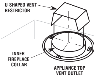
Figure 17: Vent restrictor installation—Top vent
