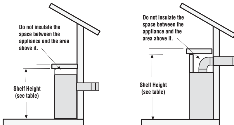
Figure 8: Shelf Height Minimum Clearances
