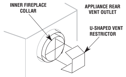
Figure 18: Vent restrictor installation—Rear vent
