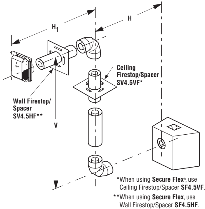
Figure 38: Rear Vent—TWO 90-DEGREE ELBOWS
