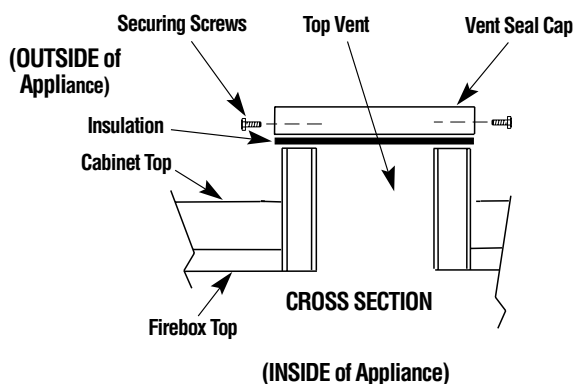
Figure 16 - TOP VENT SEAL CAP REMOVAL (TOP VENT INSTALLATIONS ONLY)
