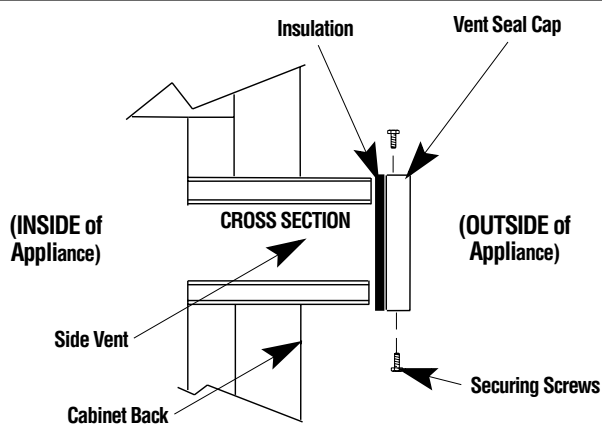
Figure 17 - SIDE VENT SEAL CAP REMOVAL (SIDE VENT INSTALLATIONS ONLY)
