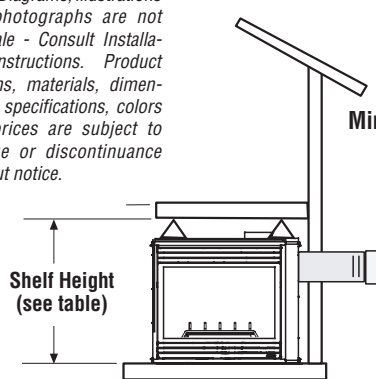
Shelf Above Fireplace With Side Venting
