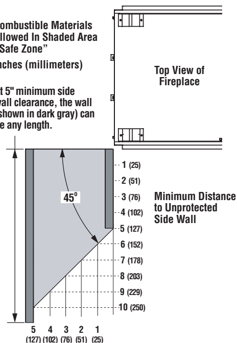
Minimum Side Clearances
