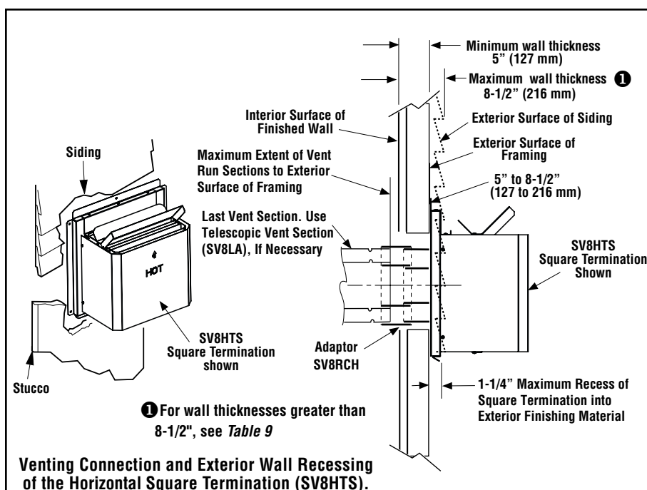
Figure 28 - Wall Thickness and Horizontal Termination Requirements
