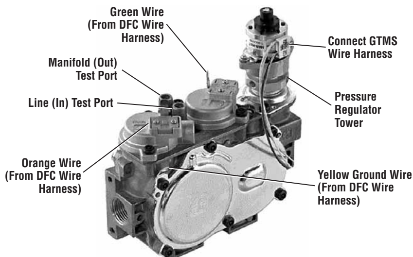
Figure 3: SIT Proflame Gas Valve
