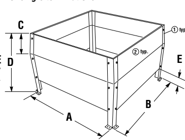
Shroud: Open Top, Chase Top - Inches (millimeters)
