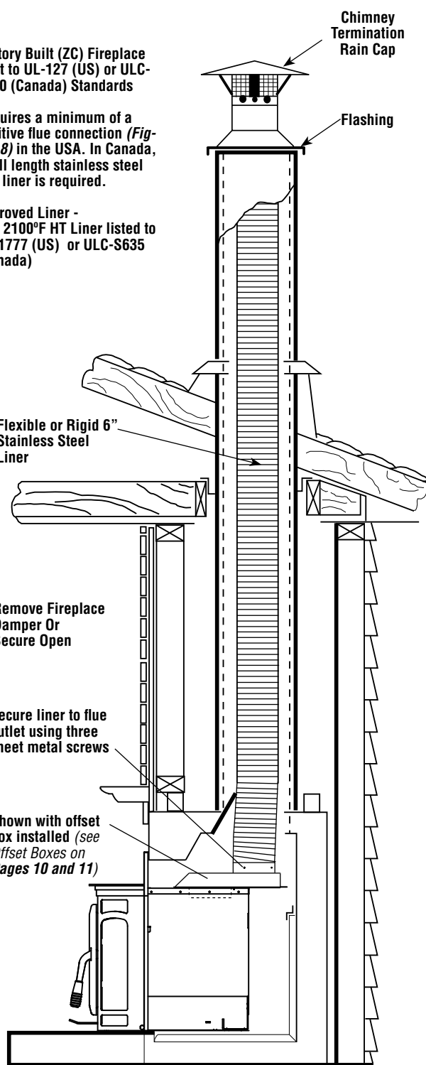
Figure 11 - Typical Installation - Factory Built Fireplace
