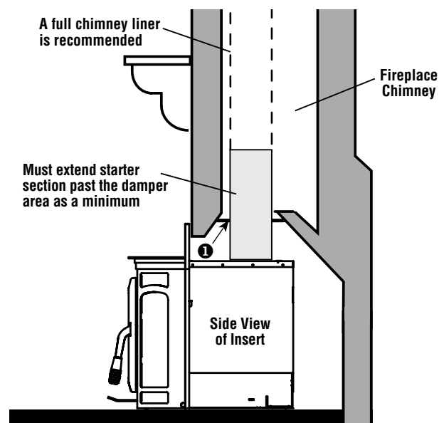
Figure 8 - Positive Flue Connection
