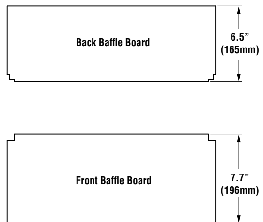
Figure 15 - Baffle Boards
