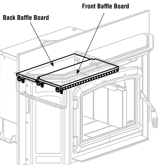
Figure 14 - Baffle Boards Installed
