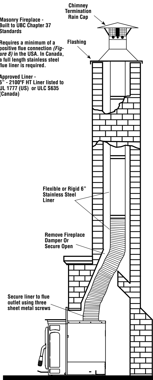
Figure 12 - Typical Installation - Masonry Fireplace
