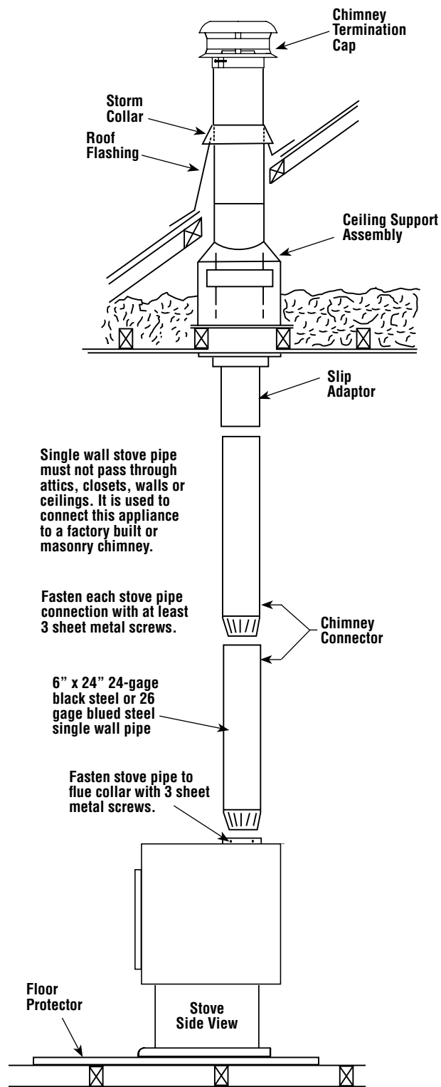
Figure 5 - Typical Installation
