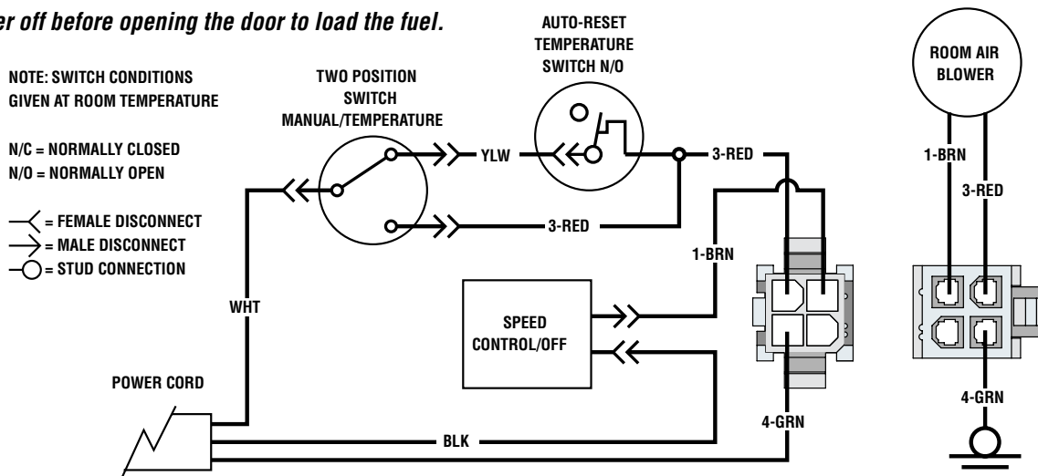
Figure 18 - Blower Wiring Schematic
