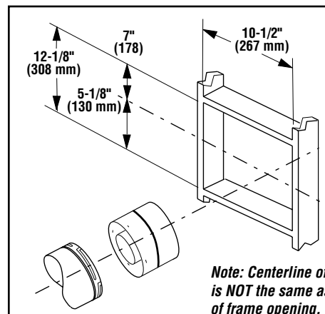
Figure 11: Exterior Wall Opening Framing
