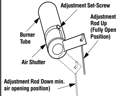
Main Burner Factory Air Shutter Opening Setting - inches (millimeter)
