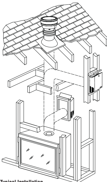
Typical Installation
