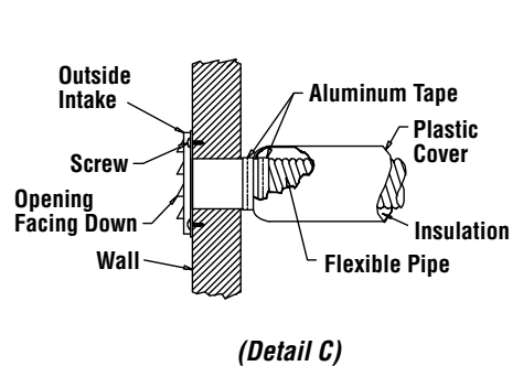
OUTSIDE AIR CONNECTION
