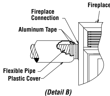
OUTSIDE AIR CONNECTION TO THE FIREPLACE
