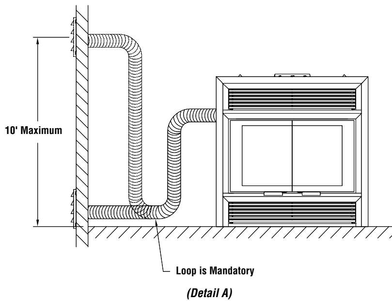
OUTSIDE AIR CONNECTION TO THE FIREPLACE
