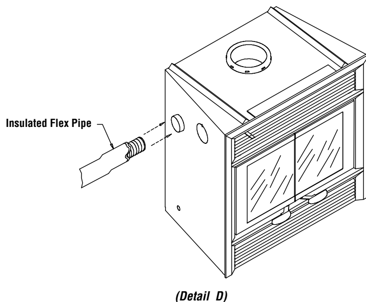
Figure 12 - External Air Intake
