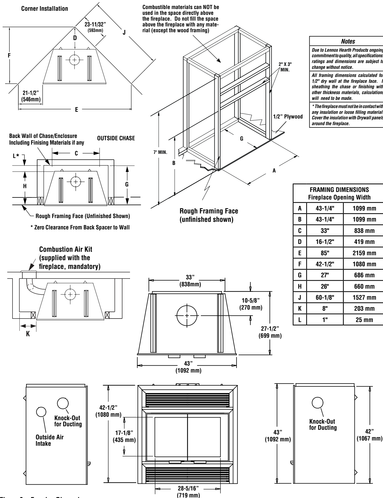
Figure 9 - Framing Dimensions
