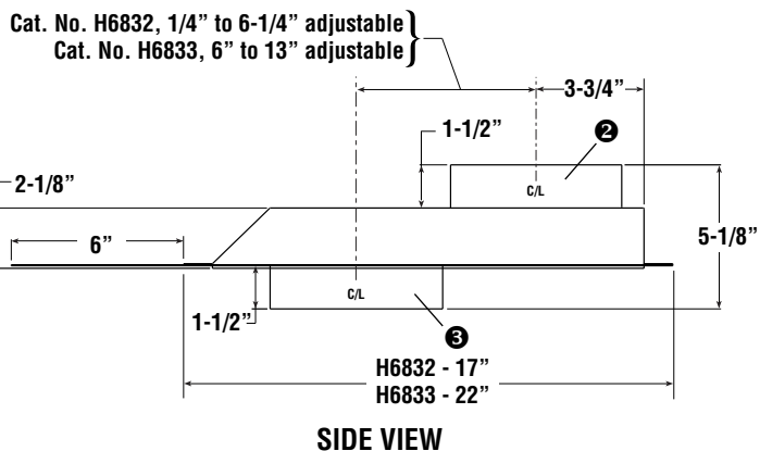
Figure 8 - Positive Flue Connection
