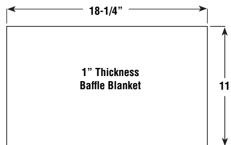
Baffle Insulation Parts
