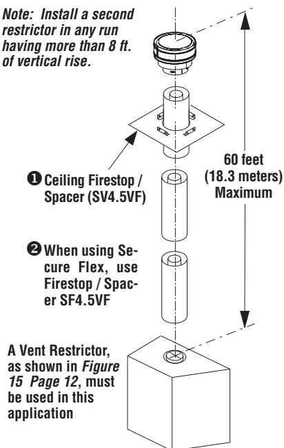
Figure 24 - Top Vent - STRAIGHT
