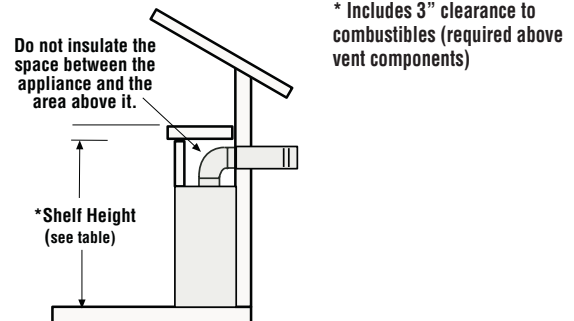
Figure 7 - Shelf Height Minimum Clearances With Top Venting
