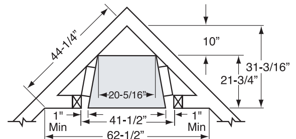
Corner Installation
