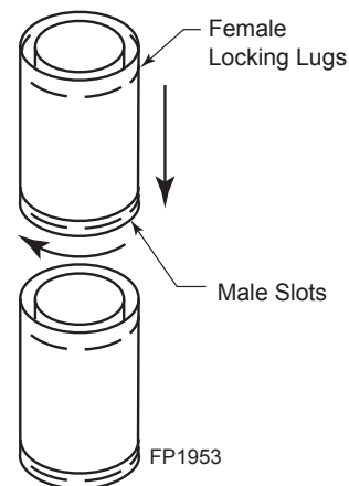
Figure 16 - Rigid Vent Pipe Connections
