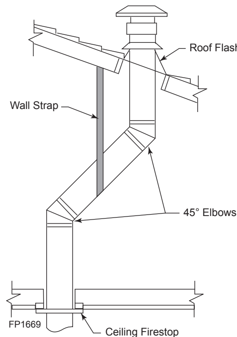
Figure 29 - Offset with Wall Strap and 45° Elbows
