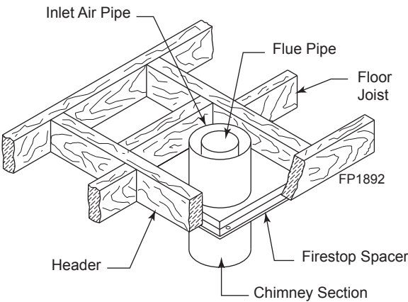
Firestop Spacer Installation at Floor Levels
