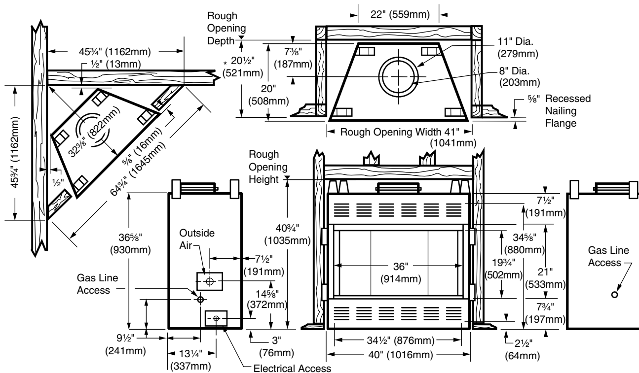
Fig. 2 BC36 Series specifications and framing.
