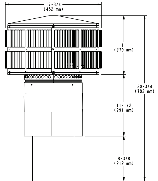
TR342-B Round Telescoping Termination Cap
