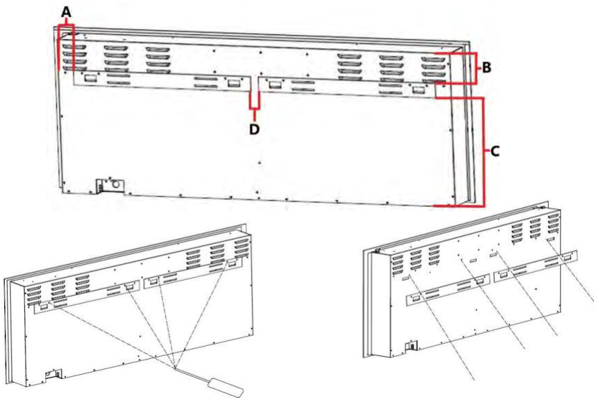
SPS-100B Wall Bracket Illustrated
